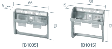
평판클립 | B1005/B1015
